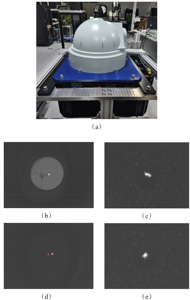
Fig. 18 Experimental verification of active detection technology: (a) laboratory imaging; (b) search and coarse track large target illumination imaging; (c) fine track large target illumination imaging; (d) search and coarse track small target illumination imaging; (e) fine track small target illumination imaging 图 18 主动探测技术实验验证: (a) 实验室成像; (b) 搜索及粗跟踪大目标照明成像; (c) 精跟踪大目标照明成像; (d) 搜索及粗跟踪小目标照明成像; (e) 精跟踪小目标照明成像
