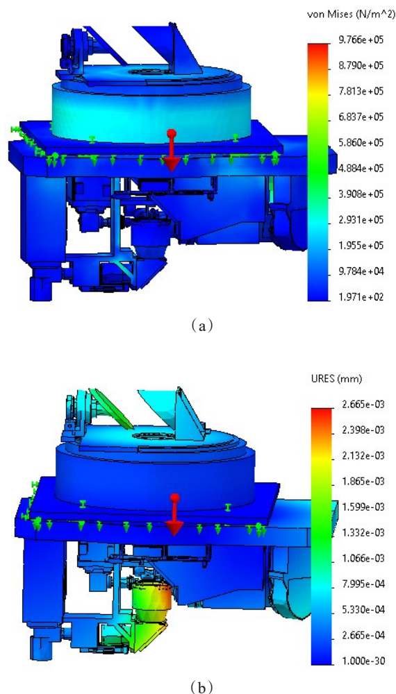
Fig. 16 Structure finite element analysis of ADMWIRSTS: (a) structural stress; (b) structural displacement
