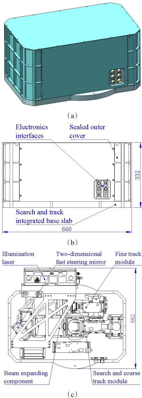
Fig. 6 Overall design of infrared search and track subsystem: (a) 3D model; (b) front view; (c) upper view (the sealed outer cover is hidden) 图6 红外搜跟分系统总体设计:(a)三维模型;(b)前视图;(c)上视图(隐藏密封外罩)
