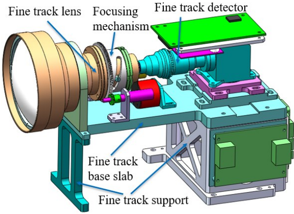
Fig. 12 Opto-mechanical structure of fine track module 图 12 精跟踪模块光机结构
