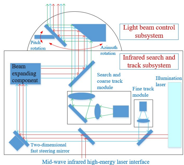
Fig. 2 Principle block diagram of active-detection mid-wave infrared search and track system (ADMWIRSTS)
