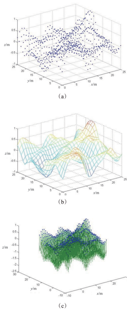
图4 激光点云波浪重构和折射修正:(a) 海表激光点云;(b) 海表轮廓拟合;(c) 激光水下载传播路径矢量 Fig. 4 Laser point cloud wave reconstruction and correction: (a) sea surface laser point cloud; (b) sea surface contour fitting; (c) underwater path vector of laser
