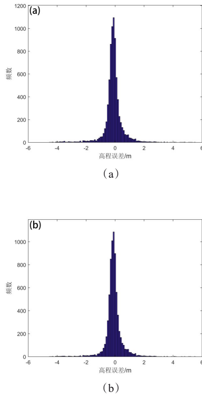
图3 资源三号03星激光测高数据筛选前后精度验证结果:(a)原始数据;(b)筛选后数据 Fig. 3 Accuracy validation results of ZY-3 03 laser altimetry data before and after screening: (a) raw data; (b) filtered data
