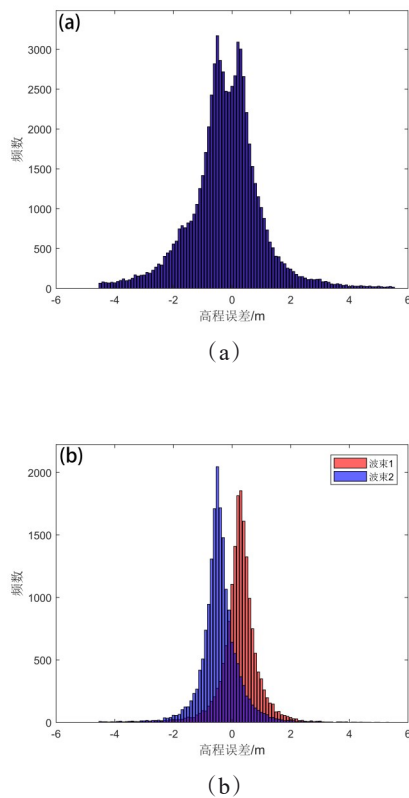
图2 高分七号激光测高数据筛选前后精度验证结果:(a)原始数据;(b)筛选后数据 Fig. 2 Accuracy validation results of GF-7 laser altimetry data before and after screening: (a) raw data; (b) filtered data
