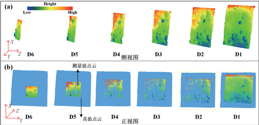
图5 (a)不同距离下混合固态激光雷达系统测量点云(侧视图);(b)测量点云与真值点云对比(正视图) Fig. 5 (a) Point clouds derived from the hybrid solid-state LiDAR system at different distances (side view); (b) comparison between the measured point clouds and the real point clouds (front view)
