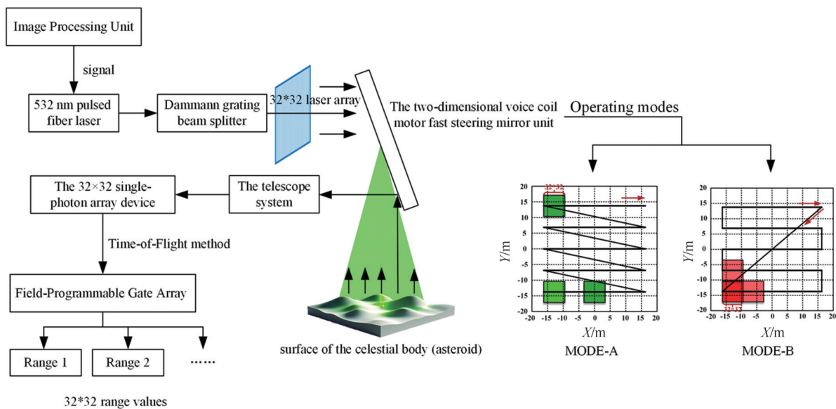
图1 混合固态激光雷达系统结构与工作模式 [14] Fig. 1 System structure and operating modes of the hybrid solid-state LiDAR system [14]
