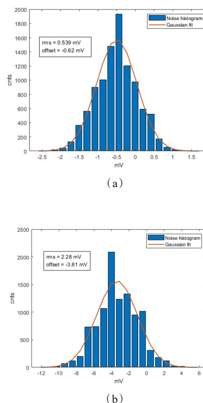
Fig. 12 The noise histogram: (a) the noise histogram of our detector; (b) the noise histogram of the commercial detector
