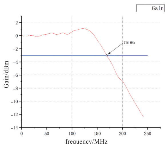
Fig. 10 ADC frequency response test
