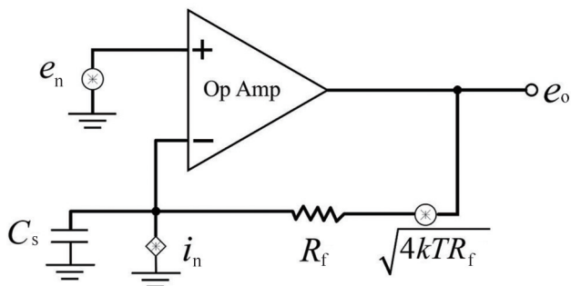
Fig. 5 Noise model of the read-out circuit 图5 读出电路的噪声模型
